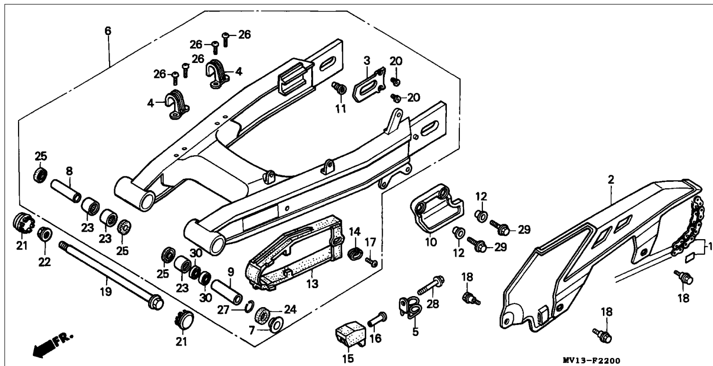
Block F-22 REAR FORK/CHAIN CASE
